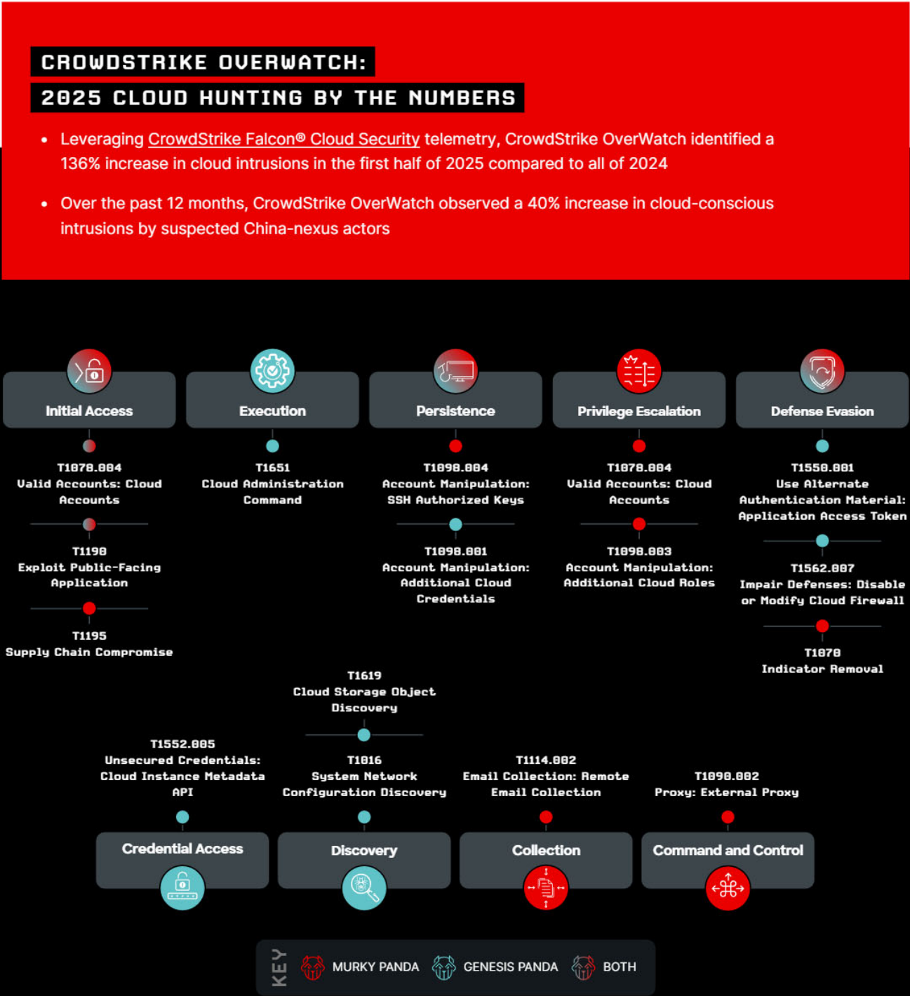
Figure 13. Prevalent MITRE ATT&CK TTPs used by MURKY PANDA and GENESIS PANDA
